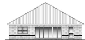
REAR ELEVATION SCALE - 1:100
