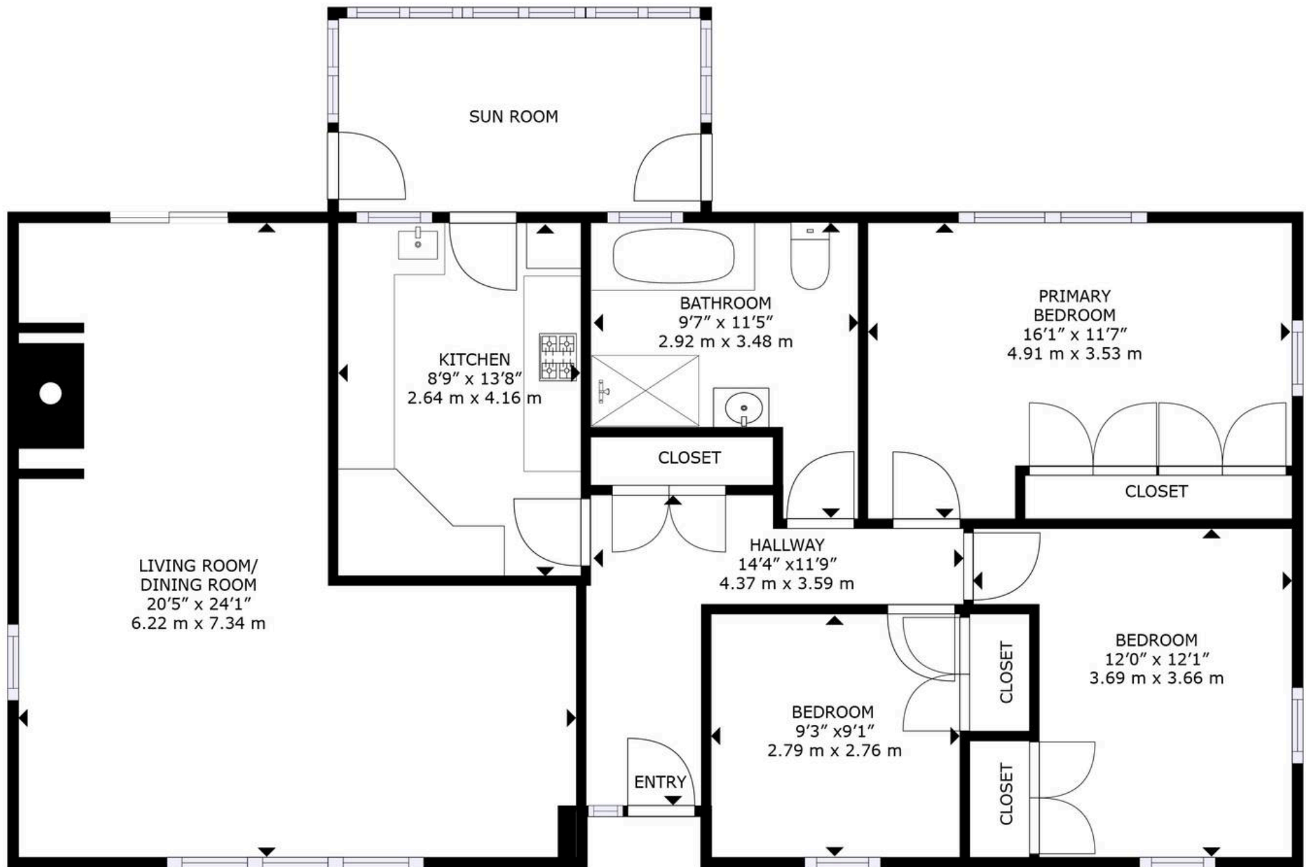
FLOOR PLAN
